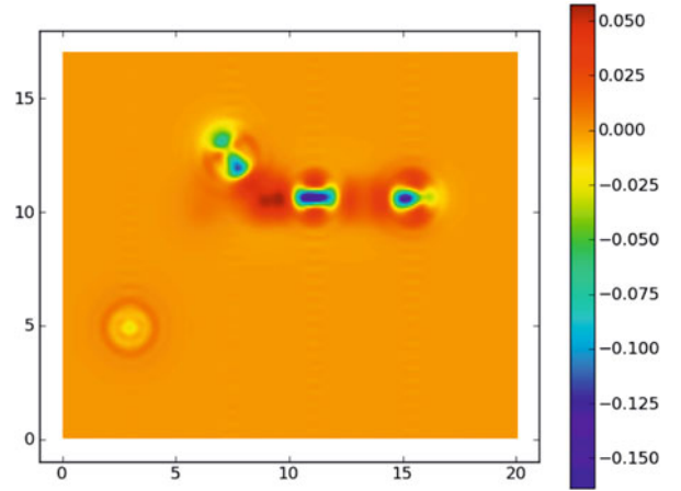
Fig. 10. (Color online) Charge redistribution \Delta\rho(r) = \rho(r) - \rho^{\text{atomic}}(r) , where \rho and \rho^{\text{atomic}} are the charges of the system after scattering and the superposition of the atomic charges of 14 non-interacting gold atoms, respectively. The \text{Au}_{13}^B atoms correspond to the horizontal blue spots, the fragmented atom is the orange-yellow circle on the lower left. The units of \Delta\rho(r) are electrons per \text{\AA}^3 .
