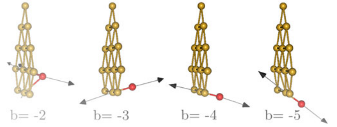
Fig. 5. (Color online) Details of the collision, with illustrations of the force vectors, for several values of the impact parameter b measured in Å units. The energy E_k = 7 eV, but the tendencies illustrated are only weakly dependent on E_k . The projectile (colored red) approaches the target from right to left. As can be seen by inspection of Figure 2 the b = -2 corresponds to fusion, b = -3 and b = -4 to fragmentation and b = -5 to scattering.
