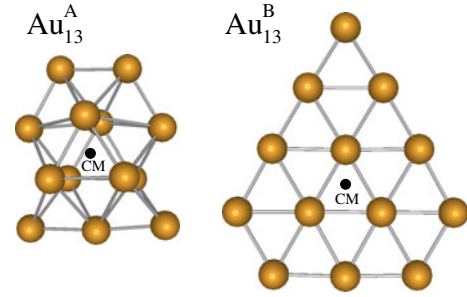
Fig. 1. (Color online) The \text{Au}_{13}^A and \text{Au}_{13}^B configurations used in our calculations. The projectile is located some distance away from the plane that is illustrated and impinges orthogonally on the target. The impact parameter b is measured in Å units relative to the cluster center of mass (CM), and is positive (negative) above (below) CM.
