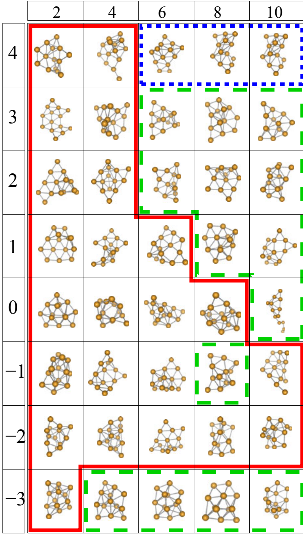
Fig. 3. (Color online) \text{Au}_{13}^{\text{A}} configurations after heat radiation. The impact parameter b , indicated at the left in Å units, is measured relative to the center of mass of the target. The kinetic energy of the projectile E_k is given at the top in eV units. The red (continuous), green (long dash) and blue (short dash) frames denote fusion, fragmentation and scattering, respectively.
