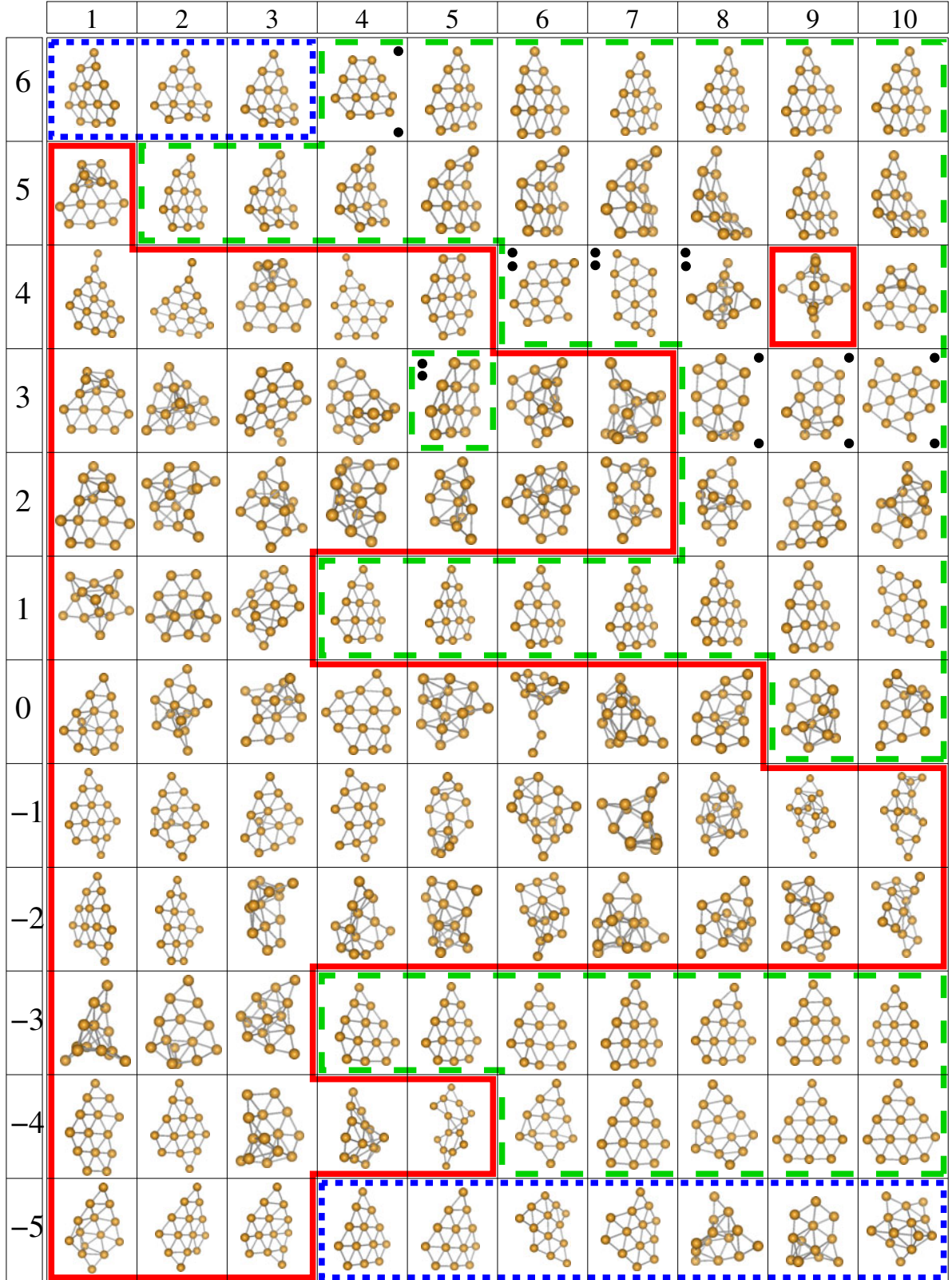
Fig. 2. (Color online) \text{Au}_{13}^B configurations after heat radiation. The impact parameter b , indicated at the left in \text{\AA} units, is measured relative to the center of mass of the target. The kinetic energy of the projectile E_k is given at the top in eV units. The red (continuous), green (long dash) and blue (short dash) frames denote fusion, fragmentation and scattering, respectively. In the fragmentation region two isolated black circles indicate that two single atoms have broken away from the cluster. Two contiguous black circles indicate that a dimer is ejected. No black circle in the fragmentation region implies the ejection of one gold atom.
